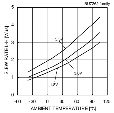
Fig.44 Slew Rate L-H – Ambient Temperature
