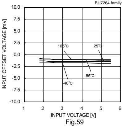
Fig.59 Input Offset Voltage – Supply Voltage (Vicm=VDD, VOUT=1.5[V])
