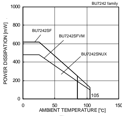
Derating curve
