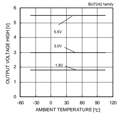
Output Voltage High – Ambient Temperature (RL=10[kΩ])
