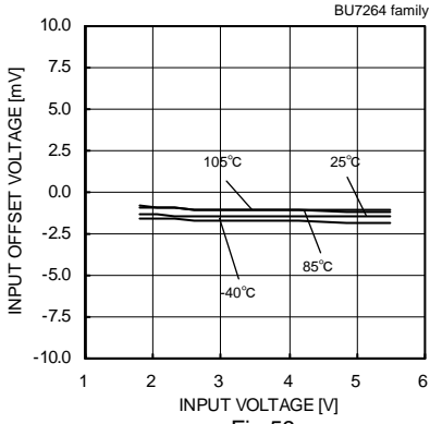
Fig.59 Input Offset Voltage – Supply Voltage (Vicm=VDD, VOUT=1.5[V])
