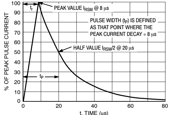
Figure 5. 8 X 20 μs Pulse Waveform
