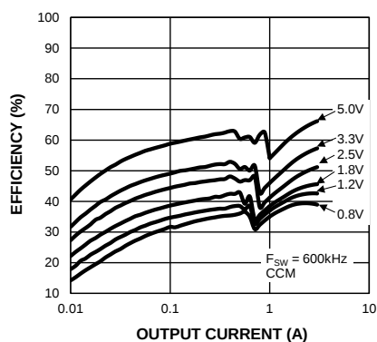
Efficiency (VIN = 70V) vs. Output Current (MIC28304-1)
