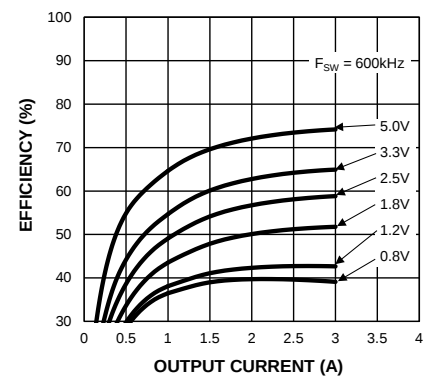
Efficiency (VIN = 48V) vs. Output Current (MIC28304-2)
