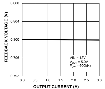
Feedback Voltage vs. Output Current (MIC28304-2)
