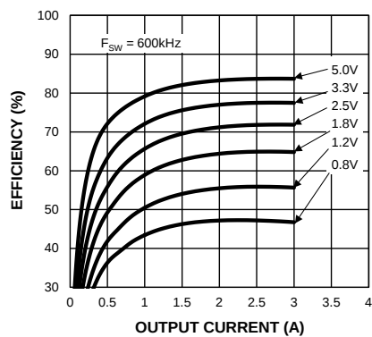
Efficiency (VIN = 24V) vs. Output Current (MIC28304-2)
