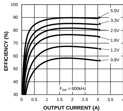
Efficiency (VIN = 12V) vs. Output Current (MIC28304-2)
