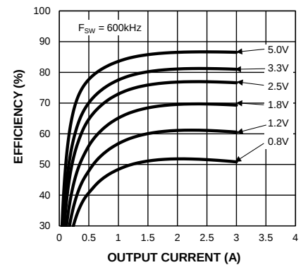
Efficiency (VIN = 18V) vs. Output Current (MIC28304-2)
