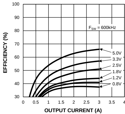
Efficiency (VIN = 70V) vs. Output Current (MIC28304-2)
