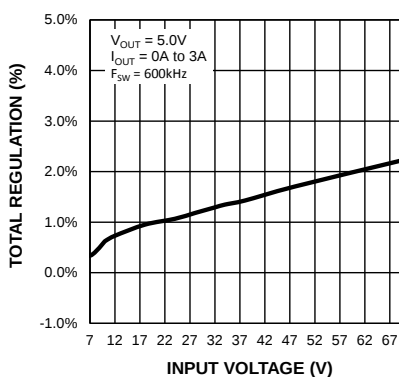
Output Regulation vs. Input Voltage (MIC28304-1)
