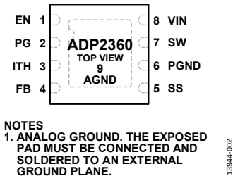
Figure 2. Pin Configuration
