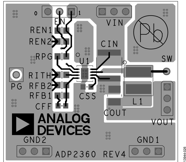
Figure 26. PCB Layout, Top
