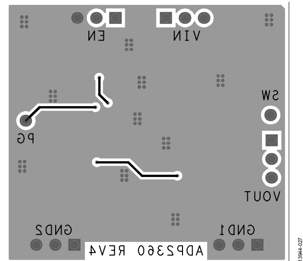
Figure 27. PCB Layout, Bottom
