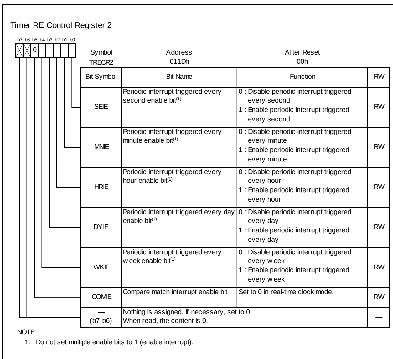
Figure 14.68 TREC2 Register in Real-Time Clock Mode
