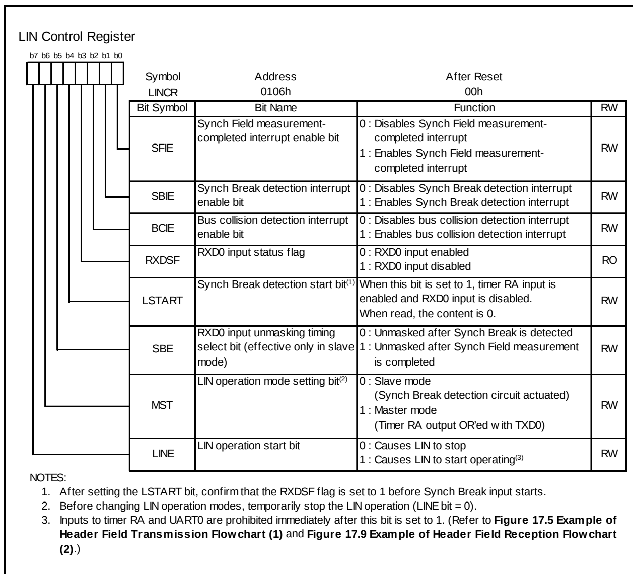
Figure 17.2 LINCX Register
