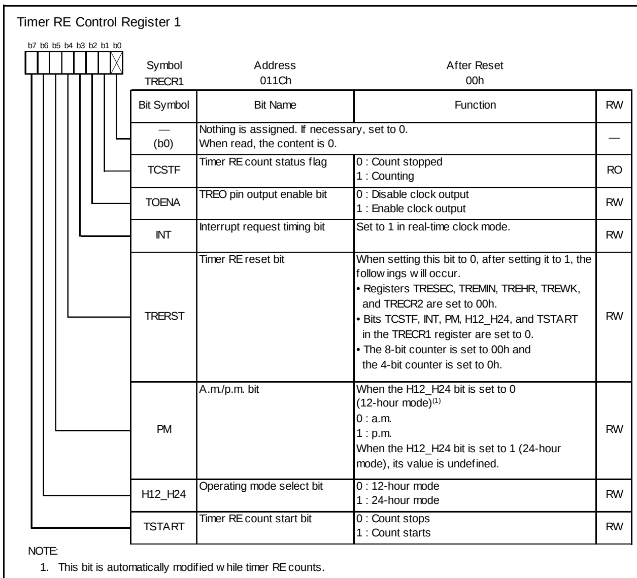
Figure 14.66 TREC1 Register in Real-Time Clock Mode
