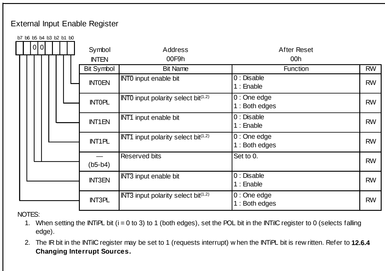
Figure 12.12 \text{INTEN} Register
