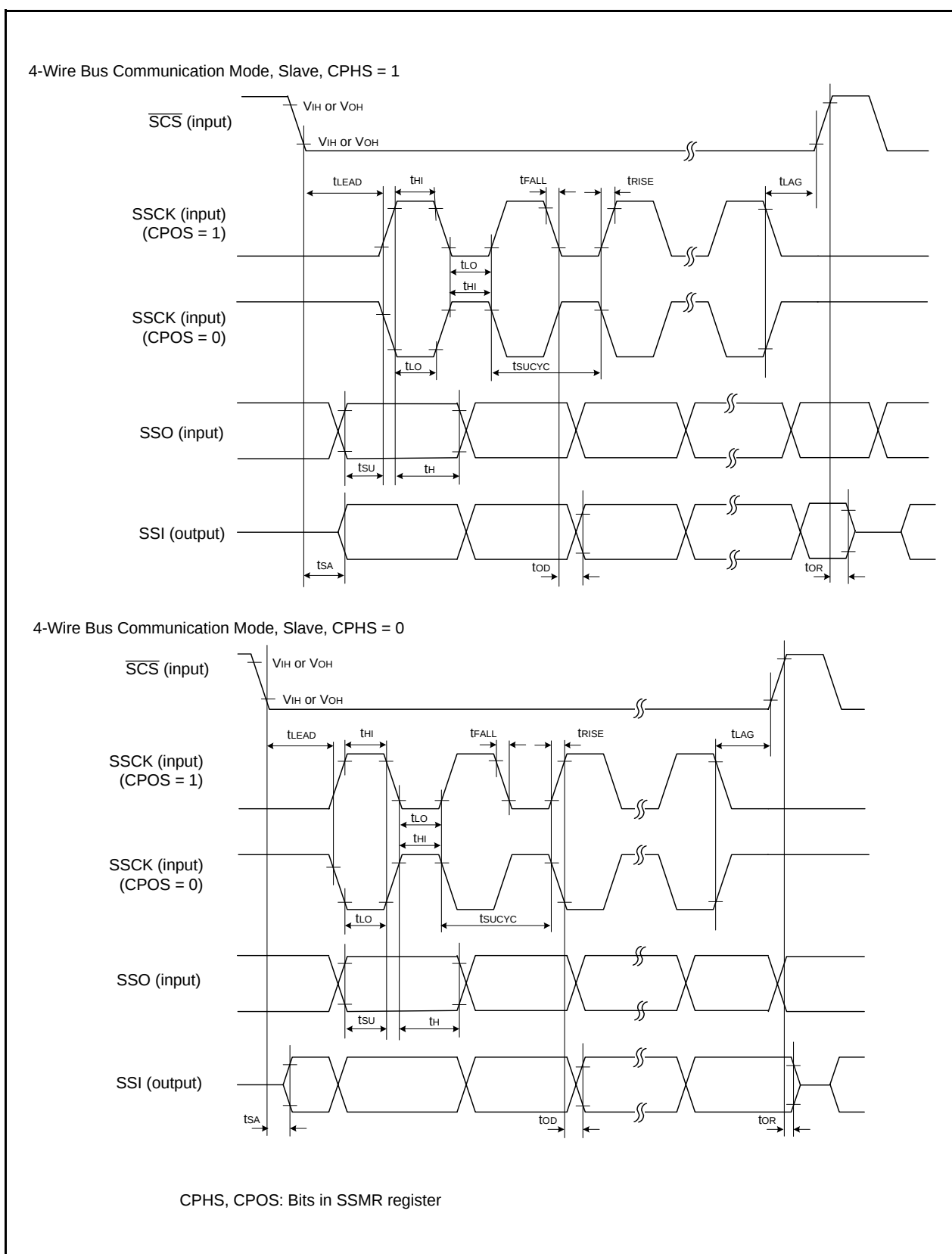
Figure 20.24 I/O Timing of Clock Synchronous Serial I/O with Chip Select (Slave)
