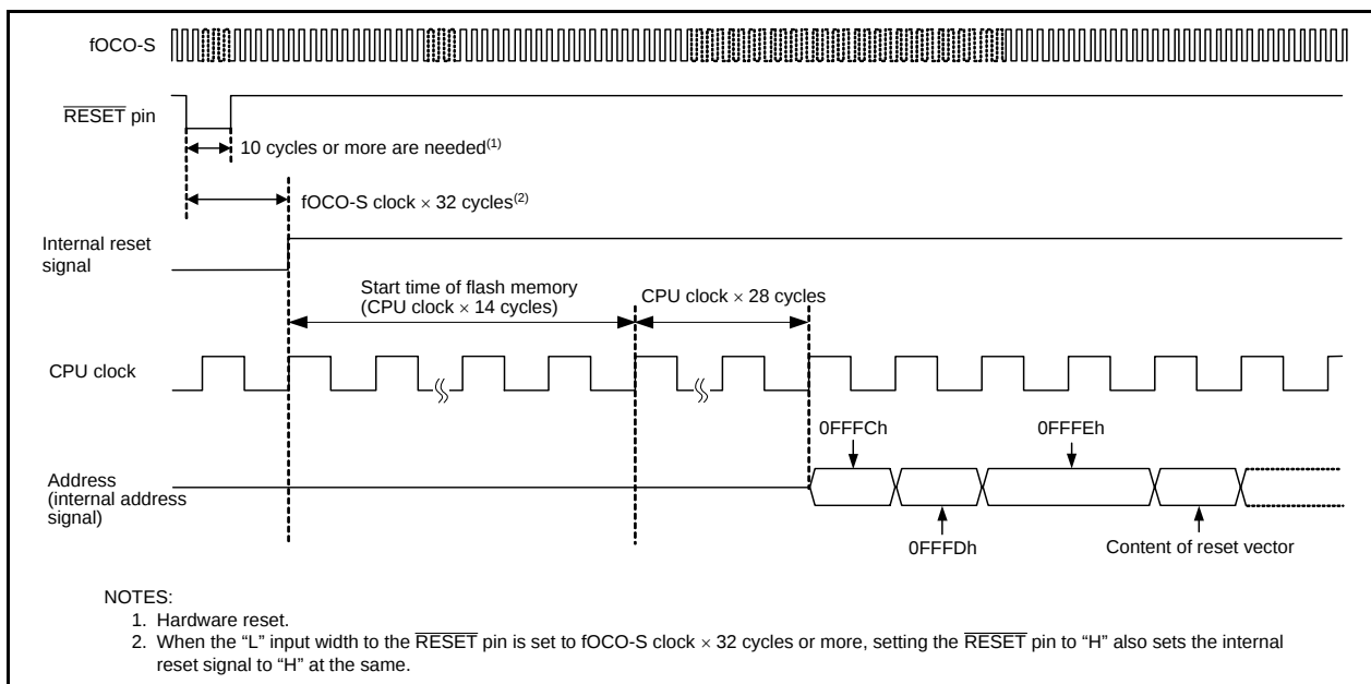
Figure 5.4 Reset Sequence
