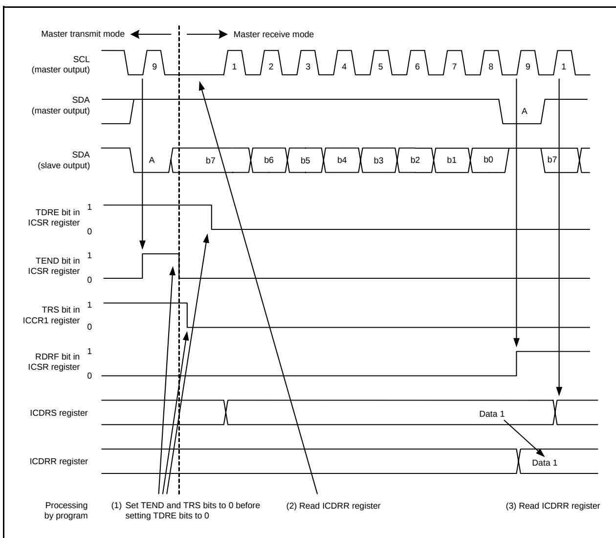
Figure 16.34 Operating Timing in Master Receive Mode (I²C bus Interface Mode) (1)
