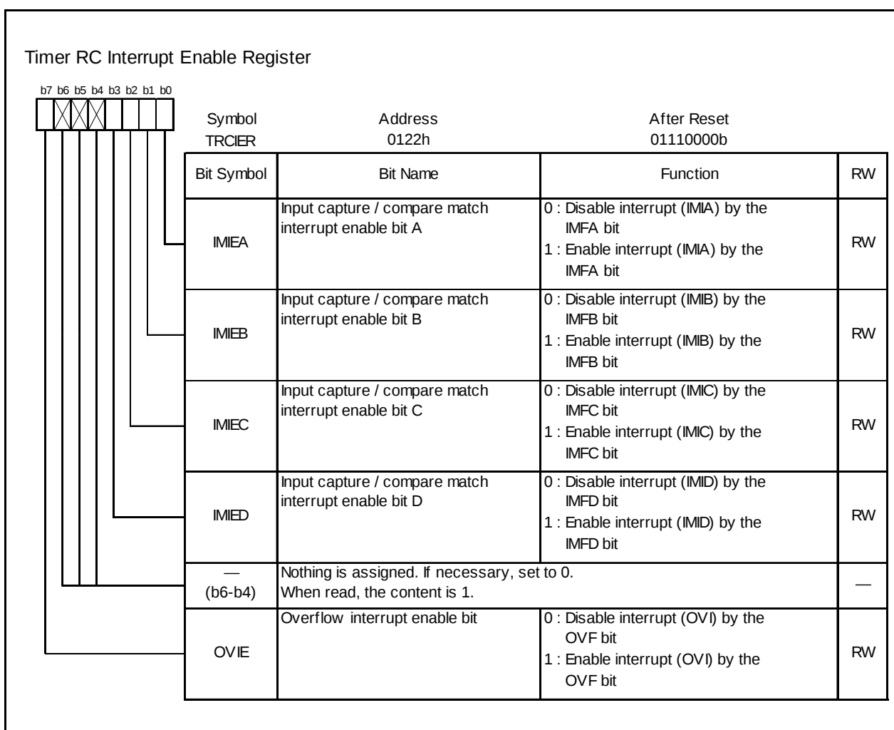
Figure 14.29 TRCIER Register
