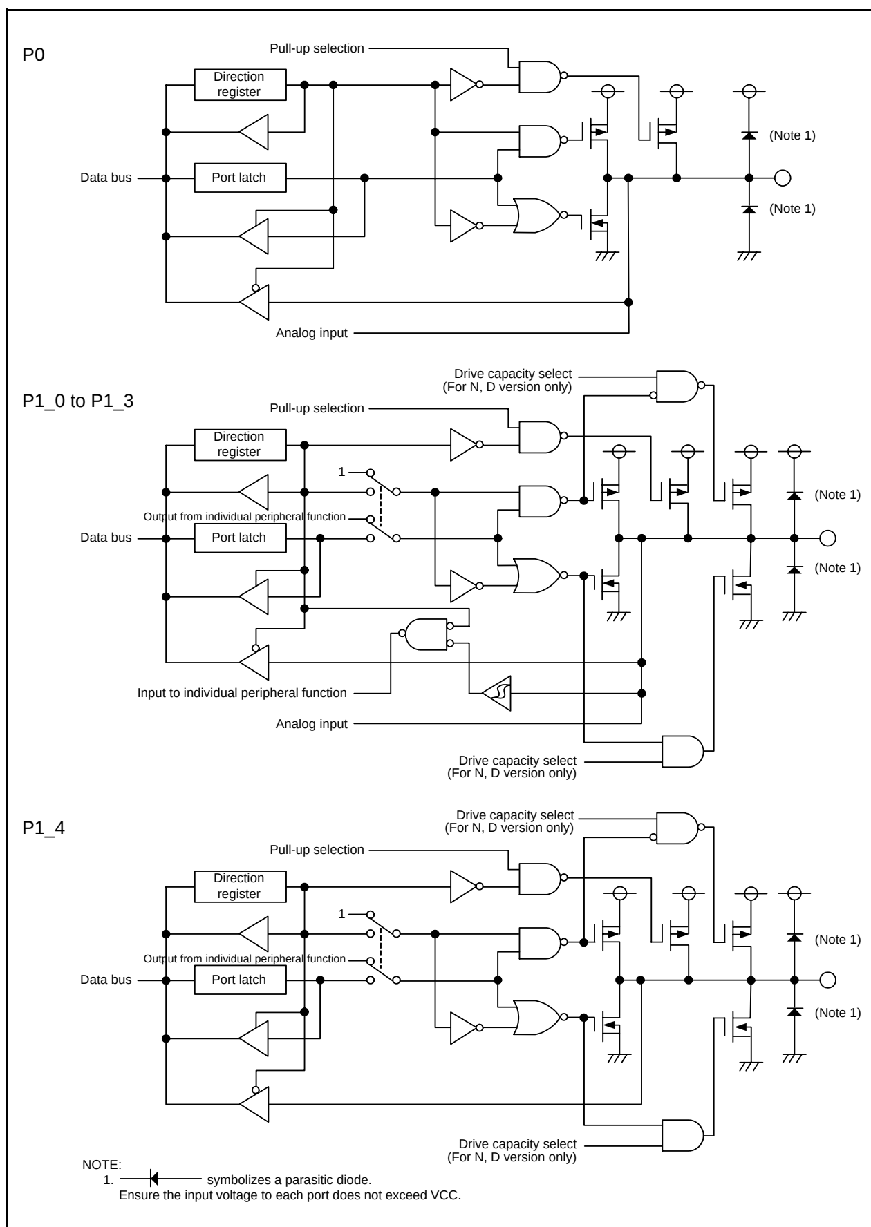
Figure 7.1 Configuration of Programmable I/O Ports (1)
