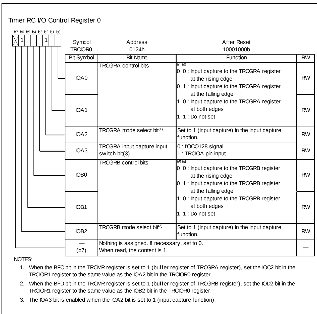
Figure 14.43 TRCIOR0 Register for Input Capture Function
