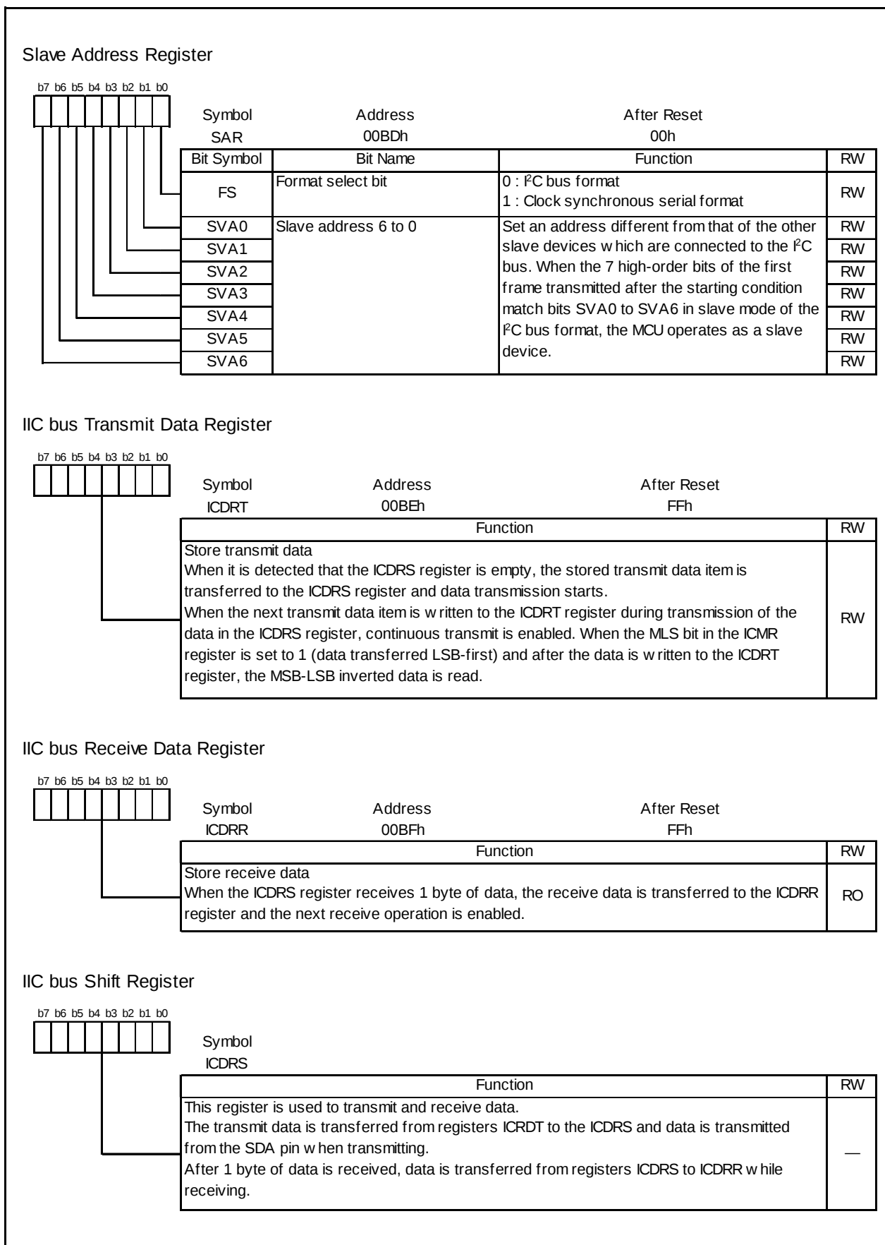
Figure 16.29 Registers SAR, ICDRT, ICDRT, and ICDRS
