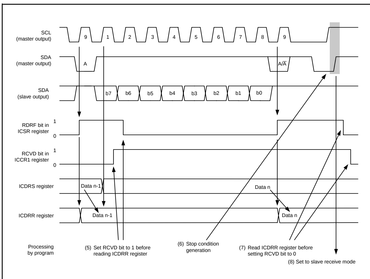
Figure 16.35 Operating Timing in Master Receive Mode (I²C bus Interface Mode) (2)
