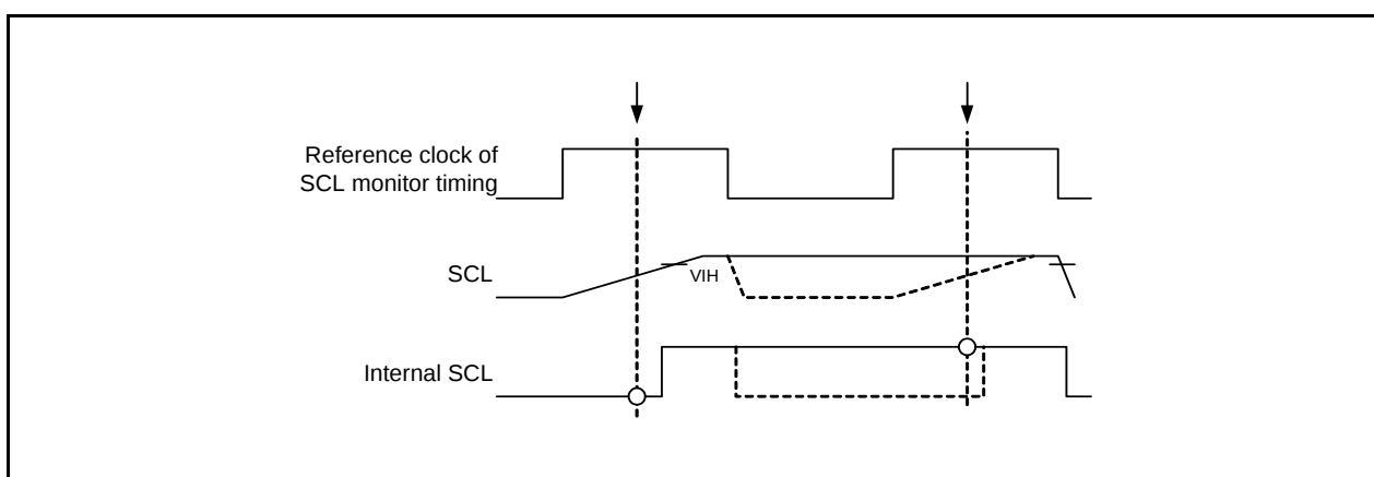
Figure 16.44 Timing of Bit Synchronization Circuit
