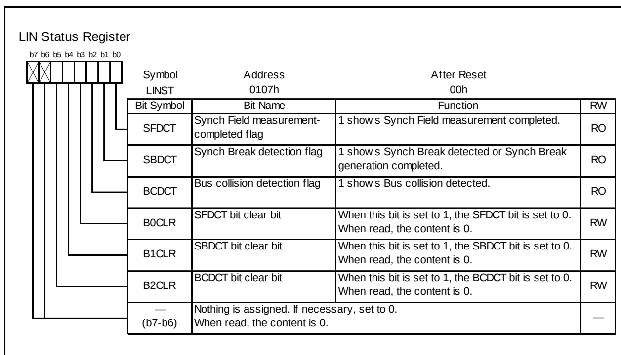
Figure 17.3 LINST Register
