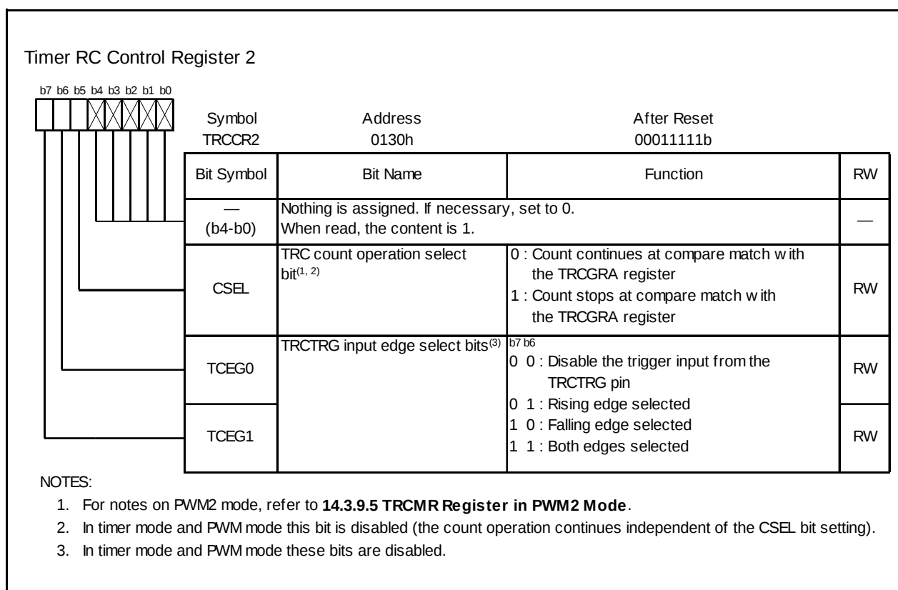
Figure 14.33 TRCCR2 Register
