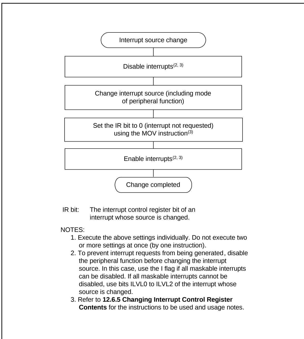
Figure 21.1 Example of Procedure for Changing Interrupt Sources
