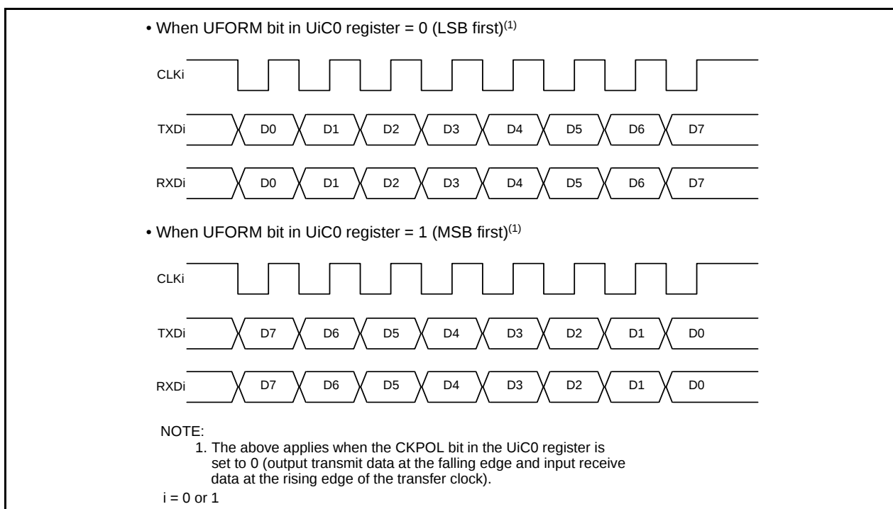
Figure 15.10 Transfer Format
