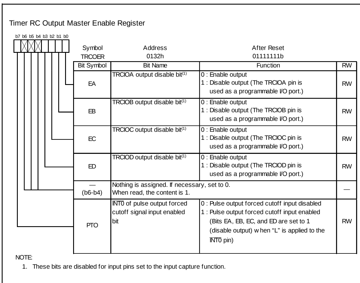
Figure 14.35 TRCOER Register
