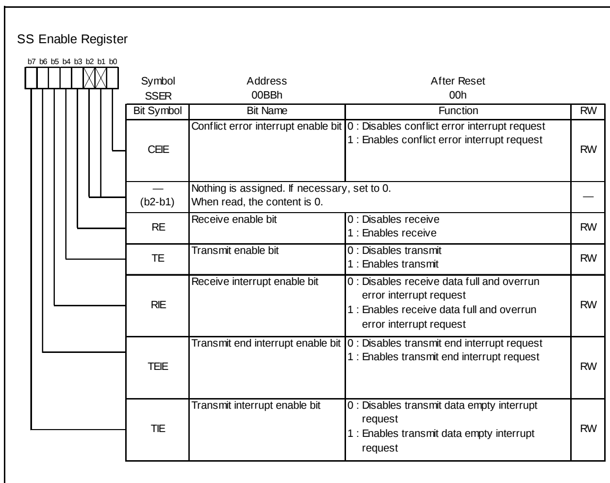
Figure 16.5 SSER Register
