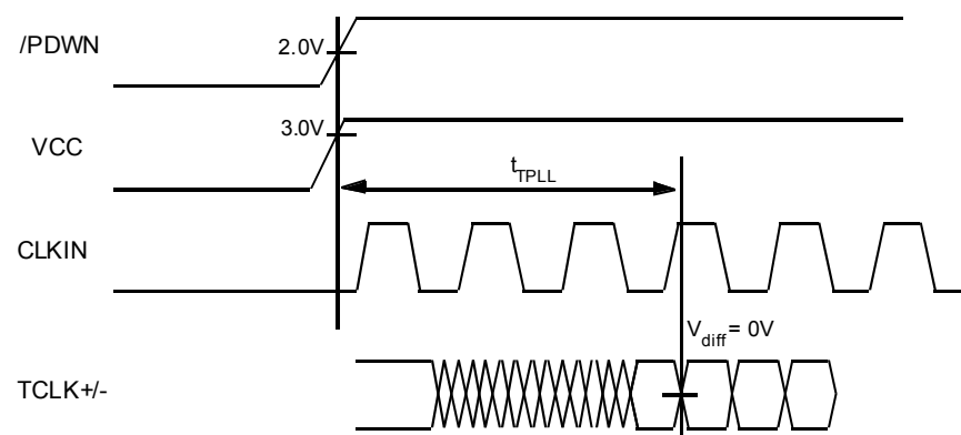
Figure 10. PLL Lock Loop Set Time
