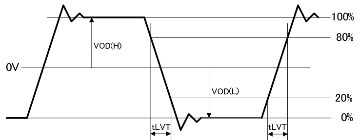
Figure 6. LVDS Output Load and Transition Time
