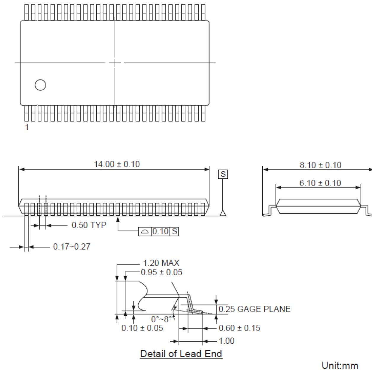
Figure 16. Package Diagram
