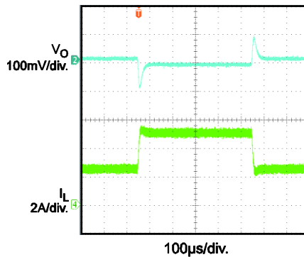
Load Transient I_O = 2.5A-5A@1.6A/\mu s
