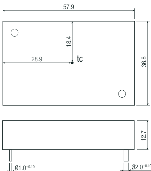
Dimension Drawing (mm)
