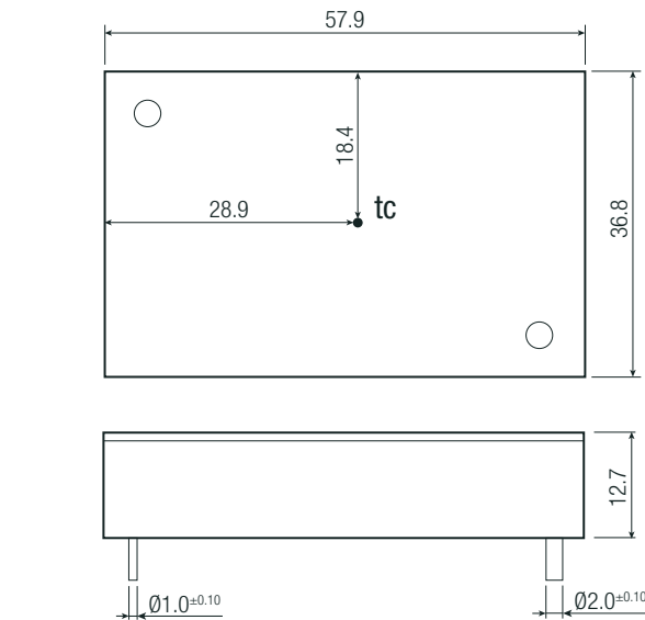
Dimension Drawing (mm)
