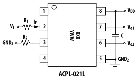
Figure 13. Recommended printed circuit board layout and input current limiting resistor selection
