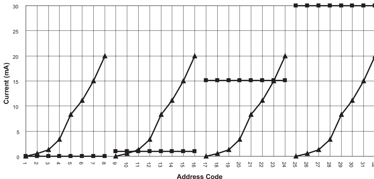
Figure 1: Output Current Level Settings (Option AAT3132).
