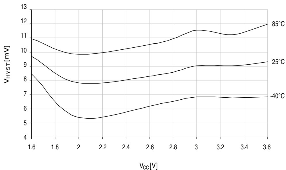
Figure 33-127. Analog comparator hysteresis vs. V_{CC} .
