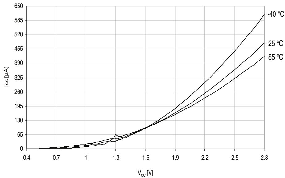
Figure 33-64. Power-on reset current consumption vs. V_{CC} .
