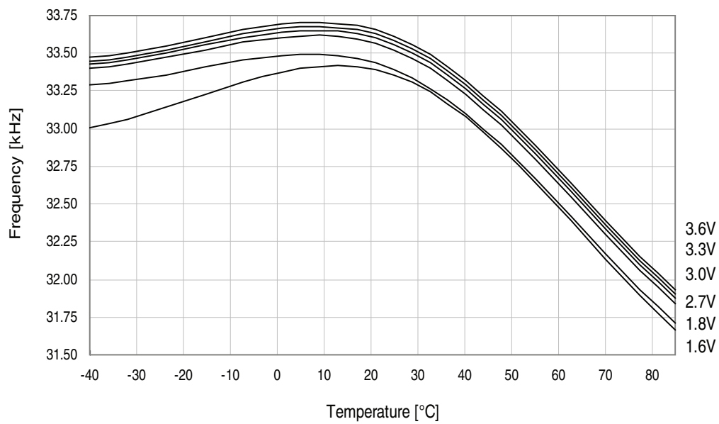
Figure 33-307. Ultra Low-Power internal oscillator frequency vs. temperature.
