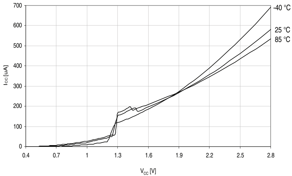
Figure 33-64. Power-on reset current consumption vs. V_{CC} .
