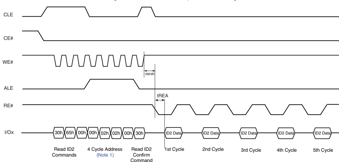
Figure 6.35 Read ID2 Operation Timing
