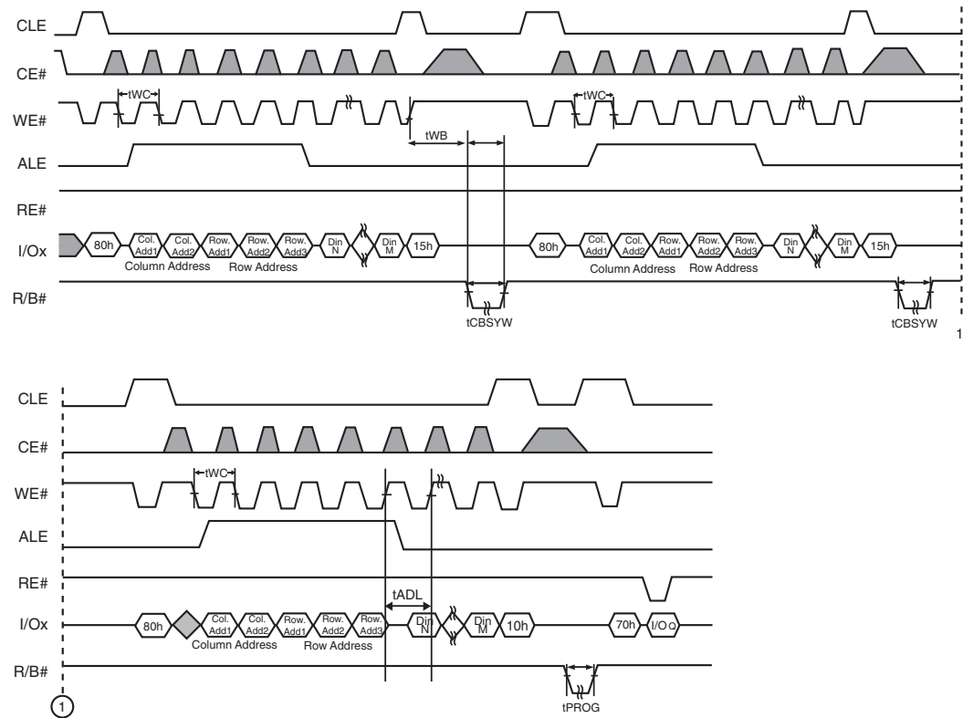
Figure 6.31 Cache Program
