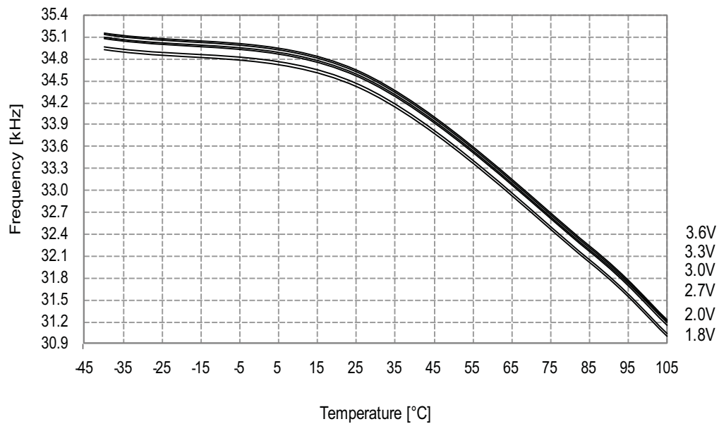
Figure 34-144. Ultra Low-Power Internal Oscillator Frequency vs. Temperature
