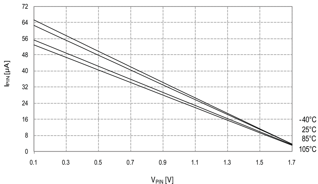
Figure 34-22. I/O Pin Pull-up Resistor Current vs. Input Voltage
