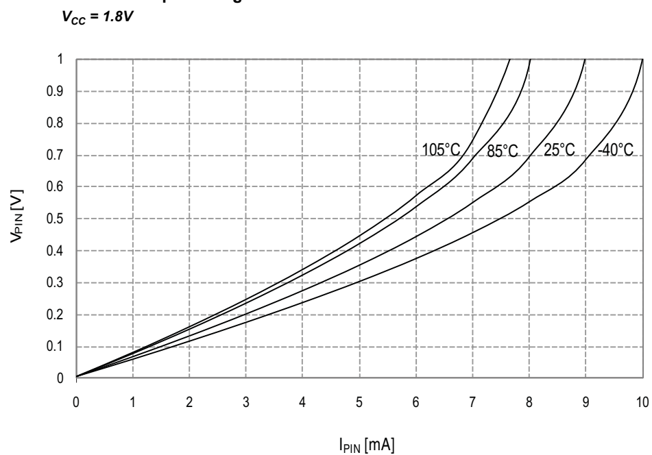
Figure 34-107. I/O Pin Output Voltage vs. Sink Current
