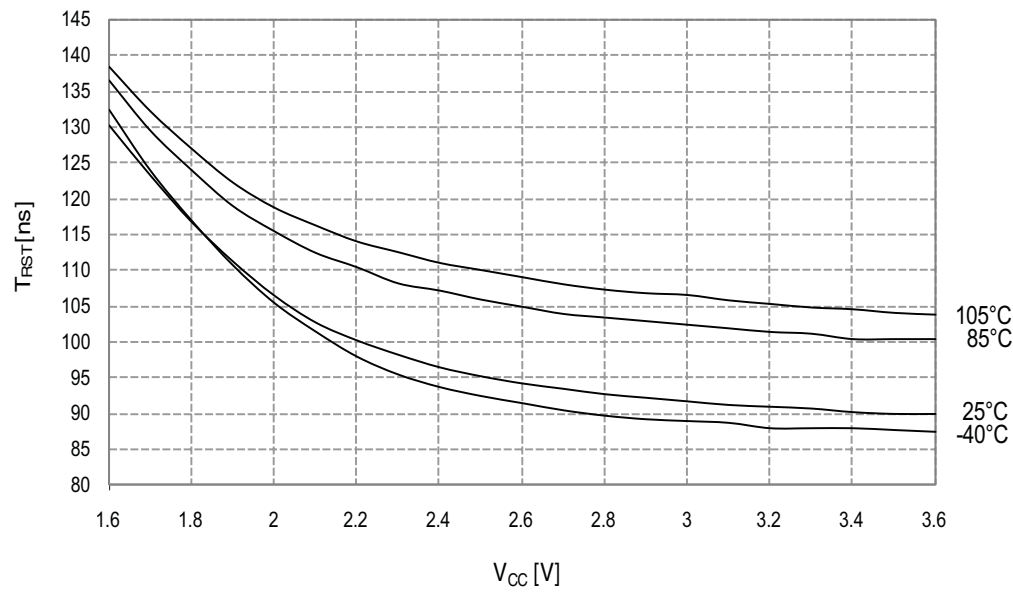
Figure 34-136. Minimum Reset Pin Pulse Width vs. V_{CC}
