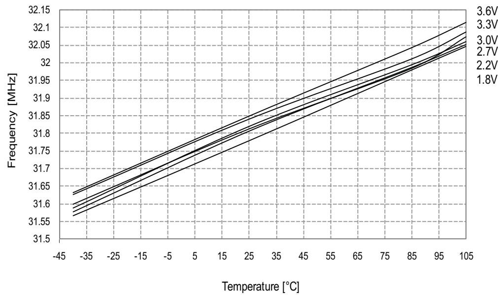
Figure 34-151. 32MHz Internal Oscillator Frequency vs. Temperature DPLL enabled, from the 32.768kHz internal oscillator
