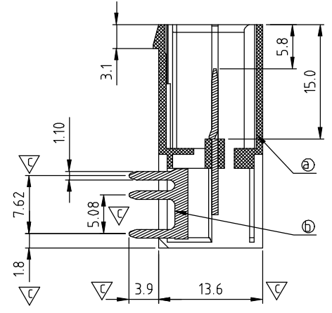
SECTION P-P
