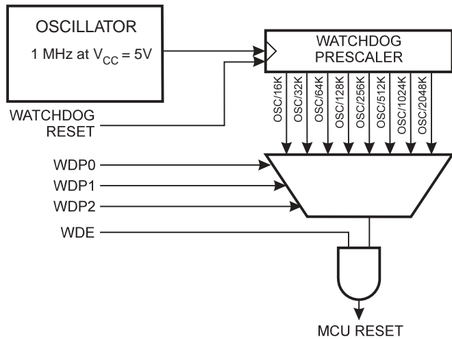
Figure 40. Watchdog Timer
