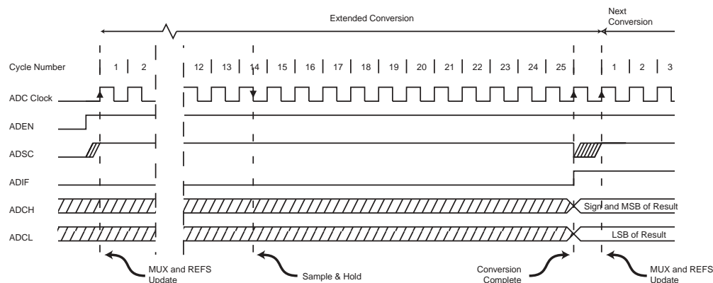
Figure 62. ADC Timing Diagram, Extended Conversion (Single Conversion Mode)
