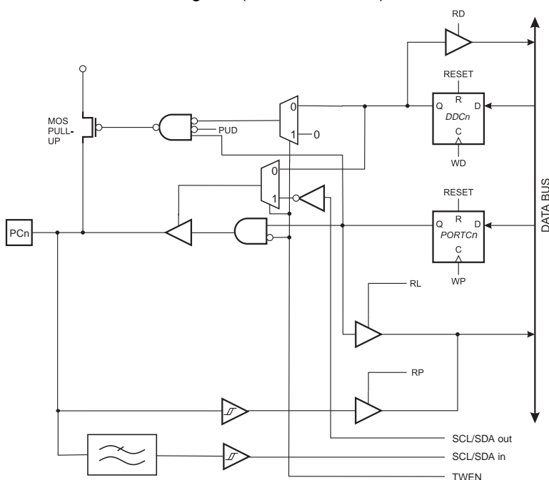
Figure 75. Port C Schematic Diagram (Pins PC0 - PC1)
