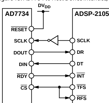
Figure 14. AD7734 to Host Device Interface, DSP
