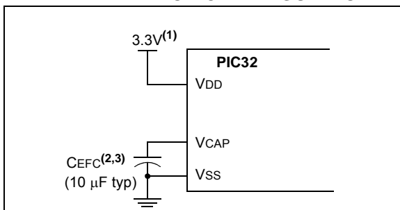
FIGURE 27-1: CONNECTIONS FOR THE ON-CHIP REGULATOR
