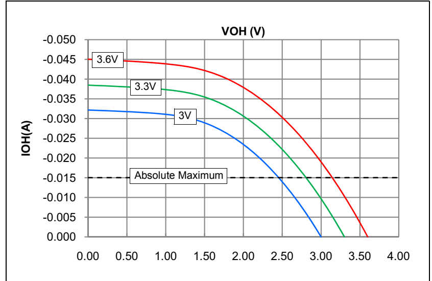
FIGURE 32-1: I/O OUTPUT VOLTAGE HIGH (VOH)
