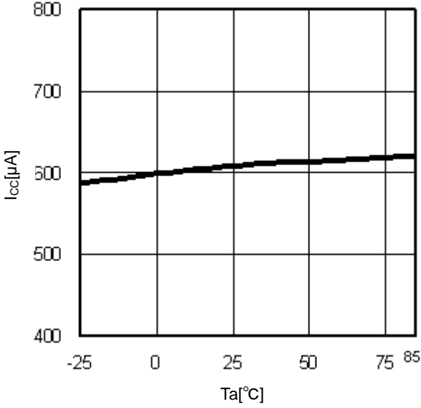
Figure 10. T_a-I_{CC}
