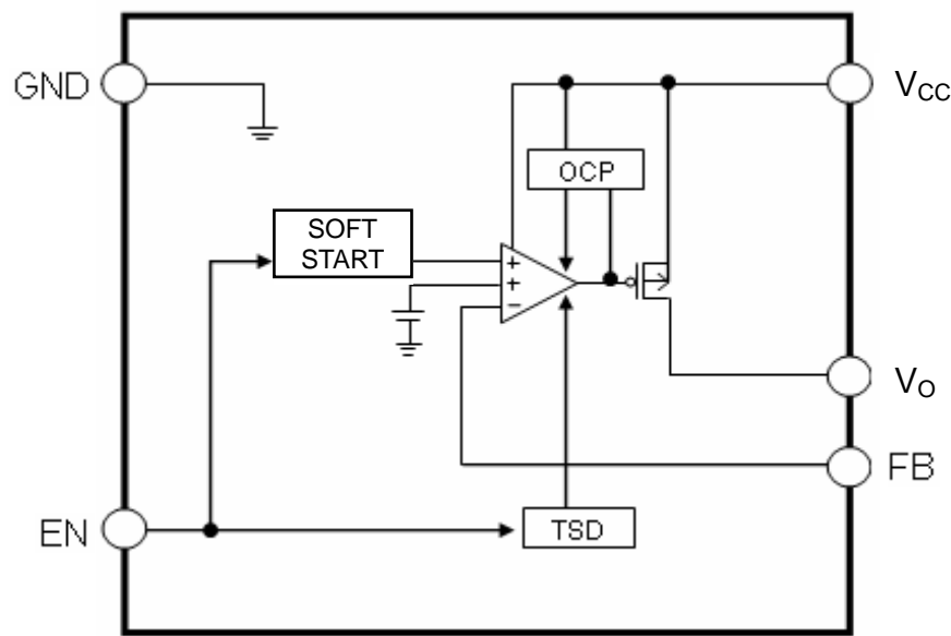
Figure 1. Block Diagram
