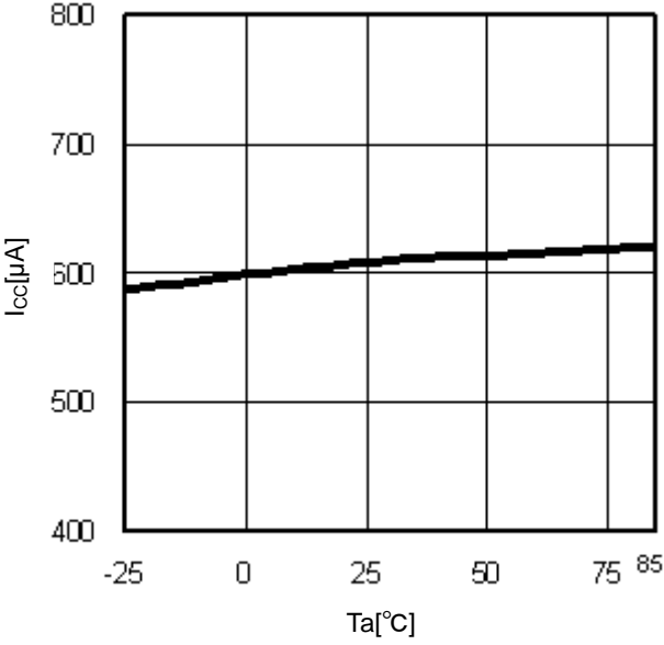
Figure 10. T_a - I_{CC}
