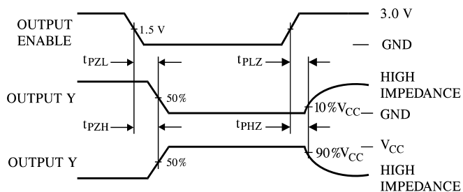
Figure 2. Switching Waveforms
