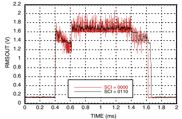
Residual Ripple for 900 MHz LTE Downlink @ SCI=0110
