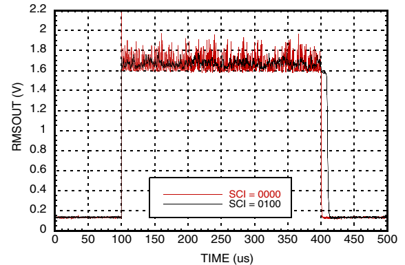
Residual Ripple for 900 MHz WCDMA4 @ SCI=0100
