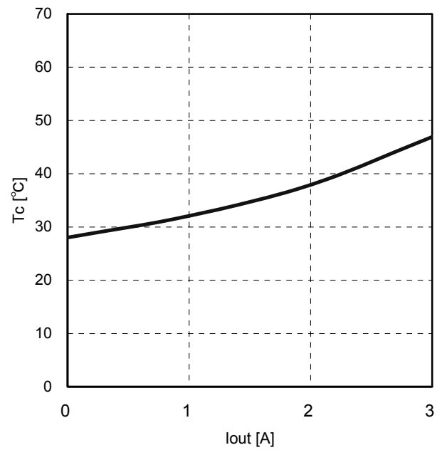
Figure 5. T_c - I_{\text{out}} ( V_{\text{IN}}=12\text{V} , V_{\text{OUT}}=3.3\text{V} , L=3.3\mu\text{H} )
