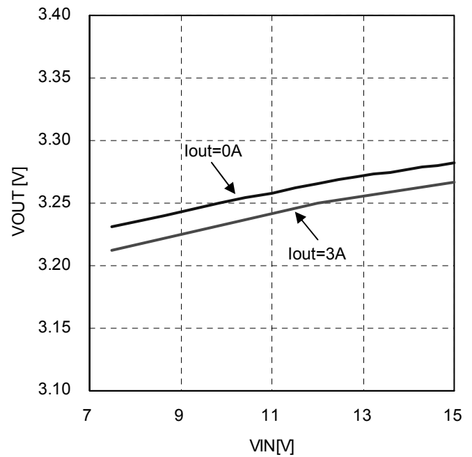
Figure 9. VOUT Line Regulation ( V_{\text{OUT}}=3.3\text{V} , L=3.3\mu\text{H} , I_{\text{out}}=0\text{A} / 3\text{A} )
