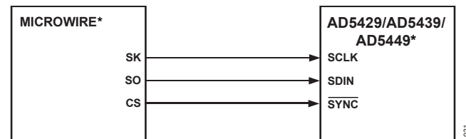
Figure 54. MICROWIRE-to-AD5429/AD5439/AD5449 Interface
