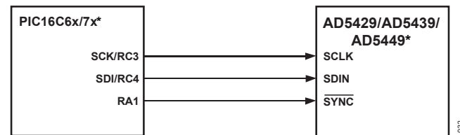
Figure 55. PIC16C6x/7x-to-AD5429/AD5439/AD5449 Interface
