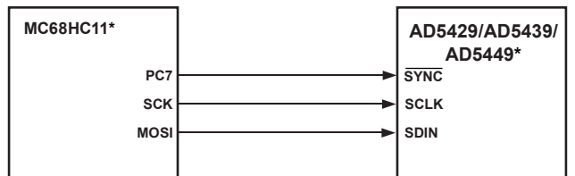
Figure 53. MCH68HC11/68L11-to-AD5429/AD5439/AD5449 Interface
