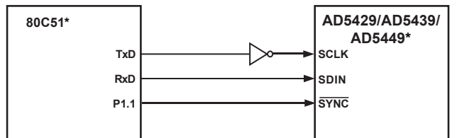
Figure 52. 80C51/80L51-to-AD5429/AD5439/AD5449 Interface
