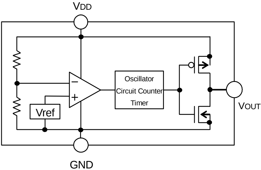
Fig.2 BU46xxxxx Series
