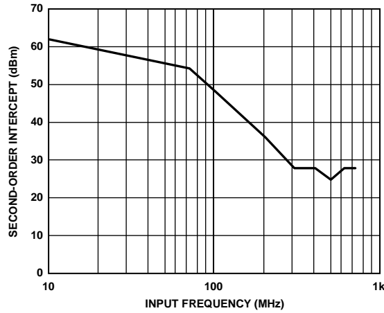
Figure 52. ADV3222 Input Second-Order Intercept, R_L = 100 \Omega , C_L = 4 pF
