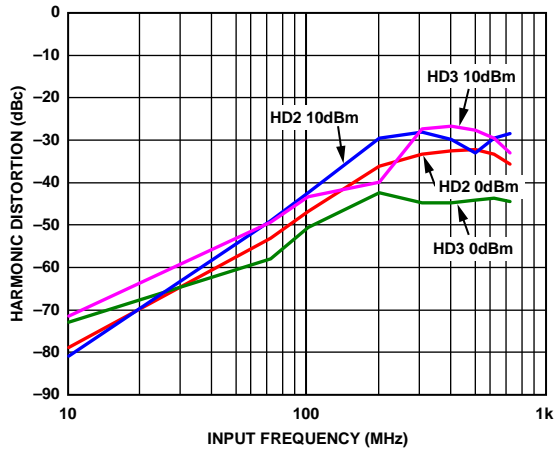
Figure 49. ADV3222 Harmonic Distortion, R_L = 100 \Omega , C_L = 4 pF
