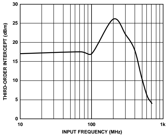
Figure 50. ADV3222 Input Third-Order Intercept, R_L = 100 \Omega , C_L = 4 pF
