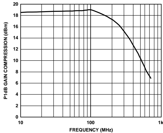
Figure 53. ADV3222 Output P1dB, R_L = 100 \Omega , C_L = 4 pF
