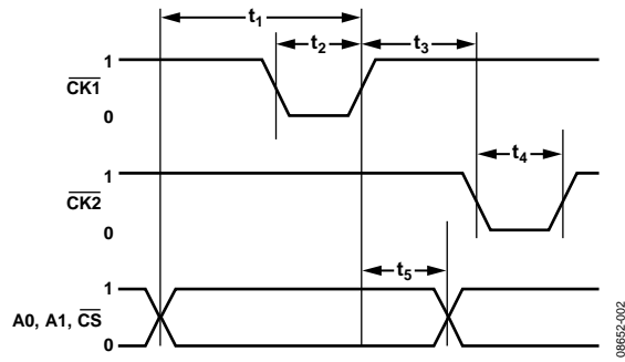
Figure 2. Timing Diagram
