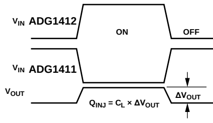
Figure 32. Charge Injection
