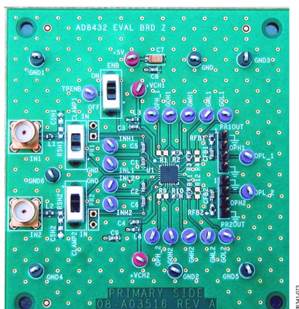
Figure 73. Evaluation Board
