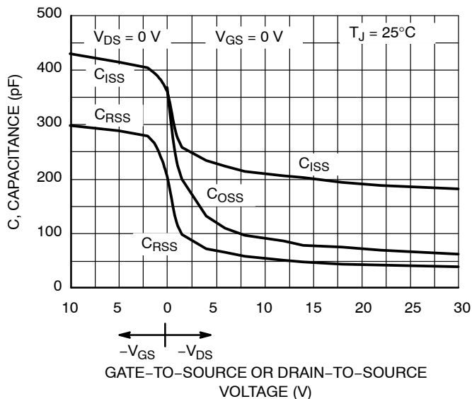
Figure 7. Capacitance Variation
