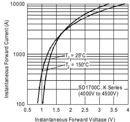
Fig. 18 - Forward Voltage Drop Characteristics
