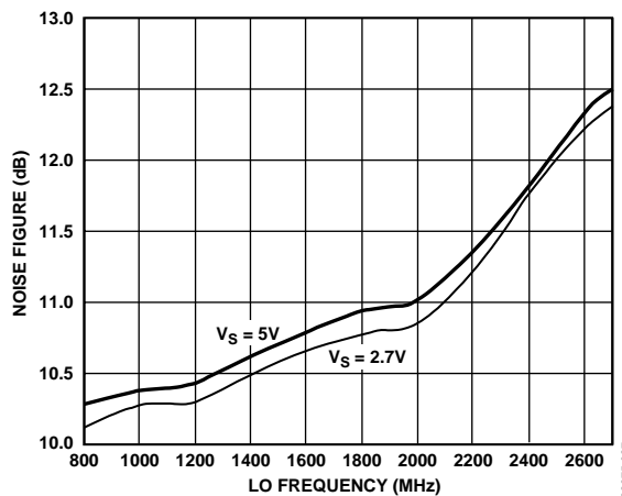
Figure 18. Noise Figure vs. LO Frequency ( F_{LO} ), Temperature = 25°C, V_{GIN} = 0.2 V, F_{BB} = 1 MHz
