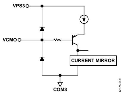
Figure 38. Circuit C
