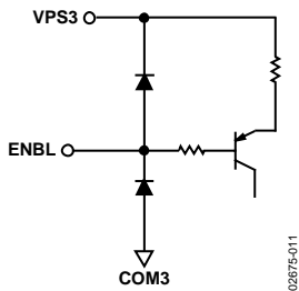
Figure 43. Circuit H
