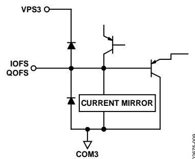
Figure 41. Circuit F
