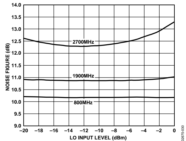
Figure 21. Noise Figure vs. LO Input Level, Temperature = 25°C, V_{GIN} = 0.2 V, V_S = 5 V
