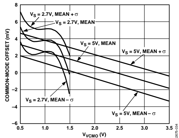
Figure 25. Common-Mode Output Offset Voltage vs. V_{CMO} , Temperature = 25^\circ\text{C} ( \sigma = 1\text{ Standard Deviation} )
