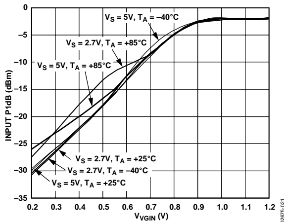
Figure 12. Input 1 dB Compression Point (OP1 dB) vs. V_{GIN} , F_{LO} = 1900 MHz, F_{BB} = 1 MHz
