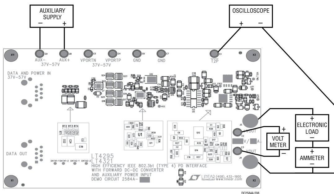
Figure 8. Setup Diagram for Auxiliary Supply Input
