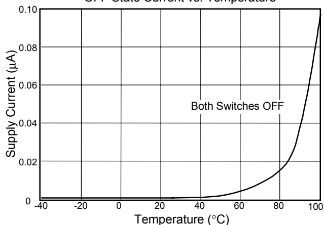
OFF State Current vs. Temperature
