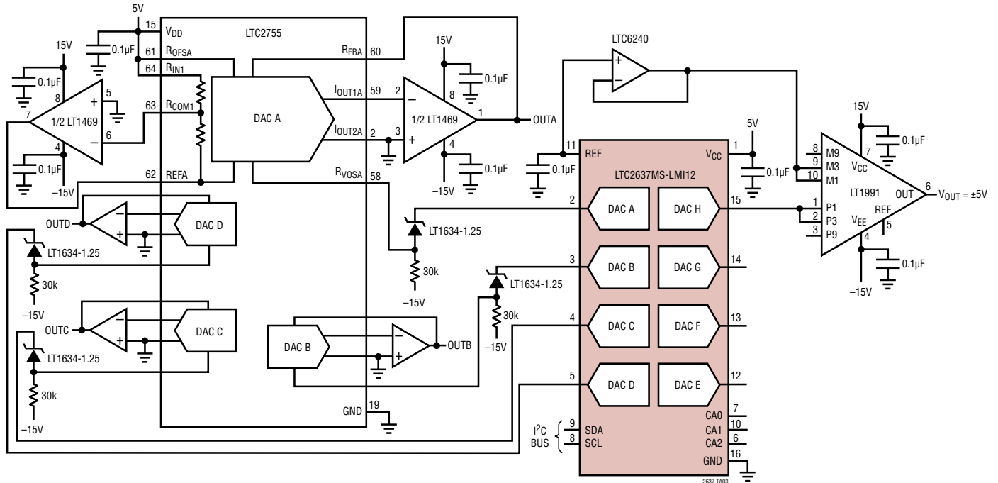
LTC2637 DACs Adjust LTC2755-16 Offsets, Amplified with LT®1991 PGA to \pm 5V
