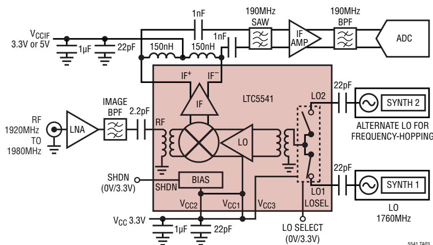
Wideband Receiver
