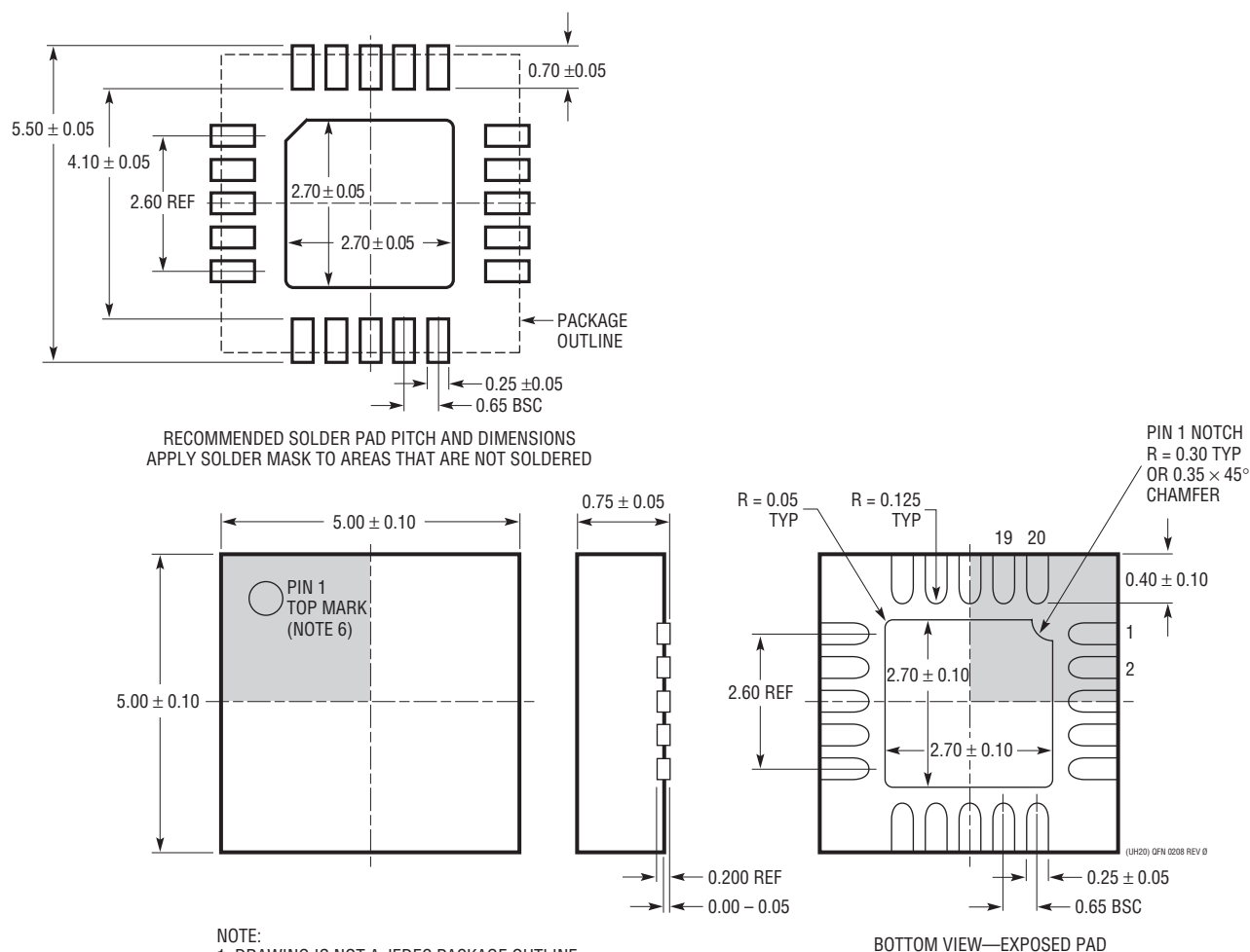
UH Package 20-Lead Plastic QFN (5mm × 5mm) (Reference LTC DWG # 05-08-1818 Rev 0)
