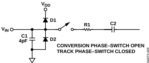
Figure 28. Equivalent Analog Input Circuit
