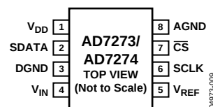
Figure 9. 8-Lead TSOT Pin Configuration
