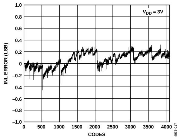
Figure 17. AD7274 INL Performance
