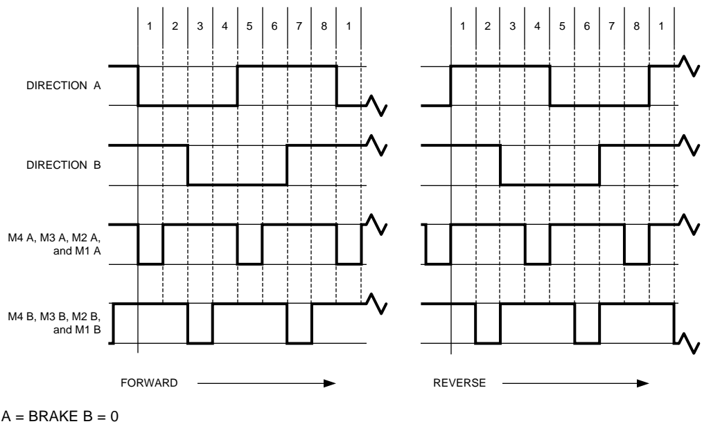
Figure 18. Winding Currents and Digital Control Signals for Half Step Drive without Torque Compensation
