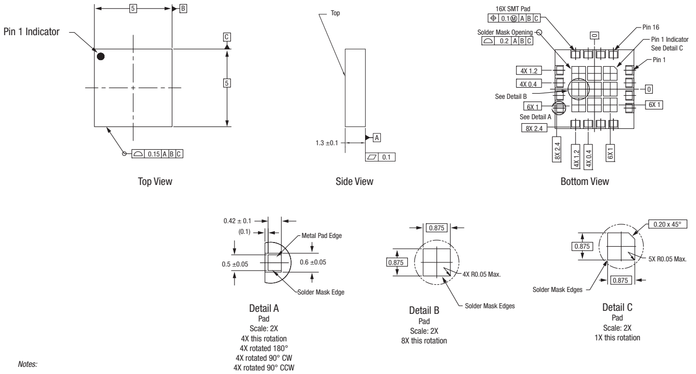
Figure 33. SKY66288-11 Package Dimensions
