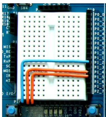
Figure 4-2 CY8CKIT-001 PSoC DVK Breadboard
