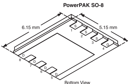
Ordering Information: SiR426DP-T1-GE3 (Lead (Pb)-free and Halogen-free)
