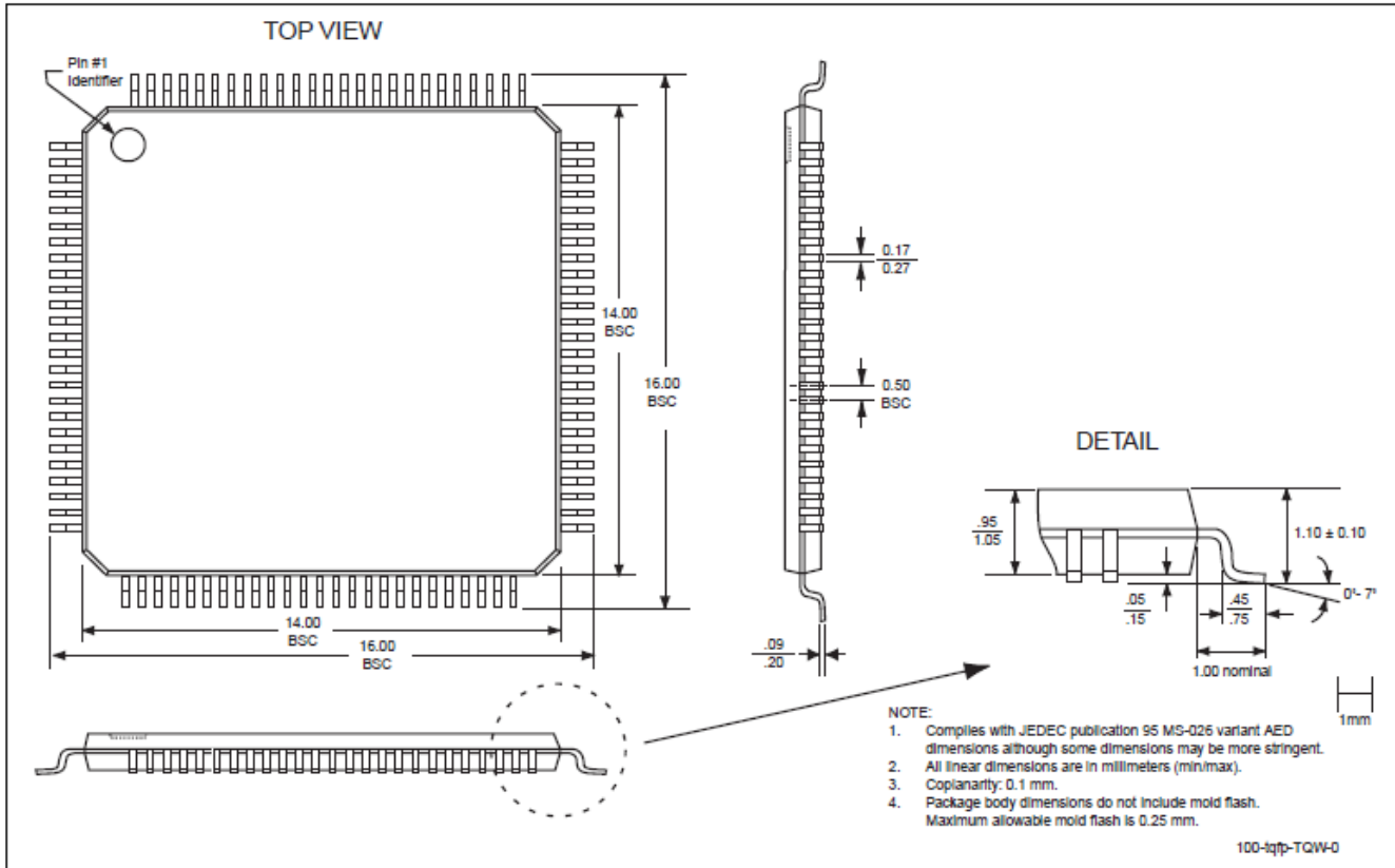
Figure 3: 100-lead Thin Quad Flat Pack (TQFP) Greenliant Package Code: TQW
