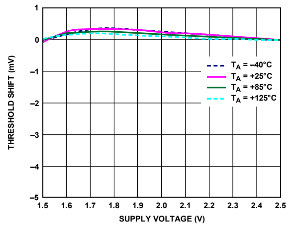
Figure 14. Minimum Supply Voltage
