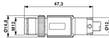
M12 SPEEDCON plug, straight
