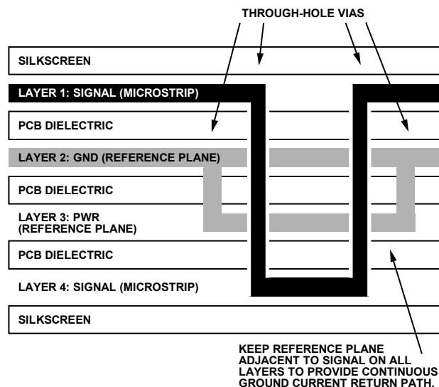
Figure 21. Example Routing of Reference Plane
