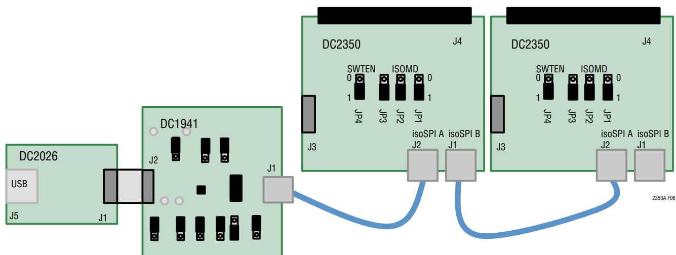
Figure 6. DC1941 Typical isoSPI Connection to the “Bottom” DC2350 in a Two-Board DC2350 Stack
