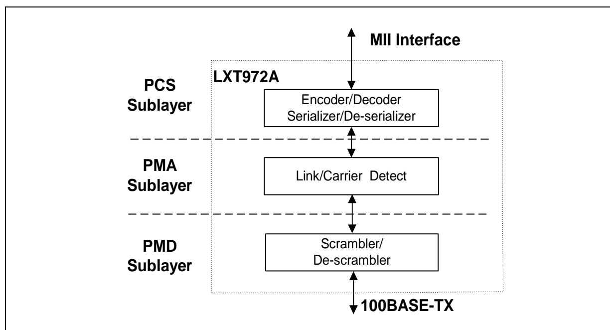
Figure 19. Protocol Sublayers
